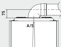
Kit coaxial orizontal Ø 60/100
